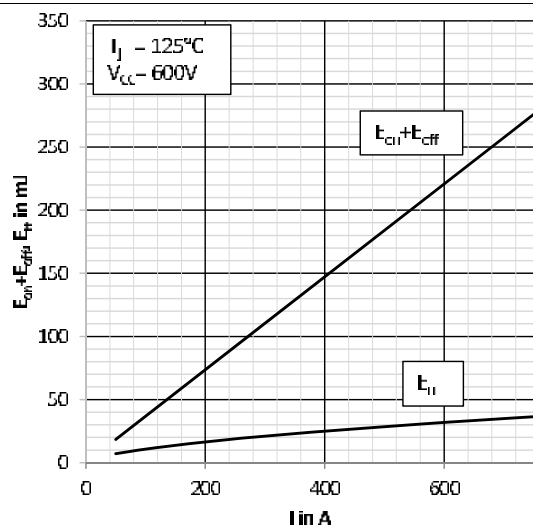
Fig. 3: Typical energy losses E = f(I_C, V_{CE})
